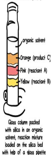
Column Chromatography
