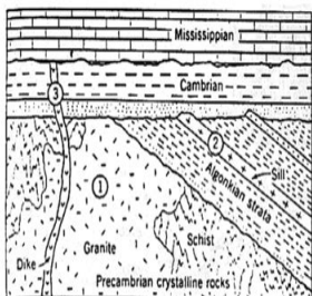
Figure 9-12: Hypothetical Geologic Cross-section Diagram
