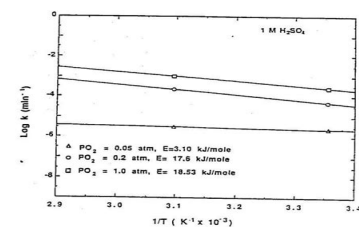
Figure 14. Arrhenius plot for the data shown in Figures 12 and 13.
