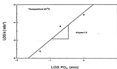
Figure 15. The order of reaction with respect to oxygen partial pressure [PO 2 ] determined for the data shown in Figure 12 at 25°C.
